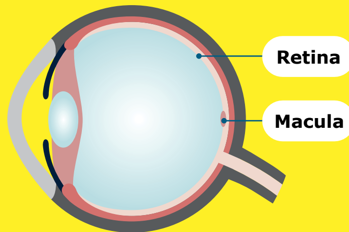
Cross-section of the eye.
